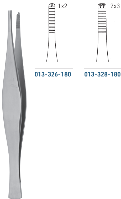
FERRIS-SMITH 013-326-180 - 013-328-180 18,0 cm / 7"
